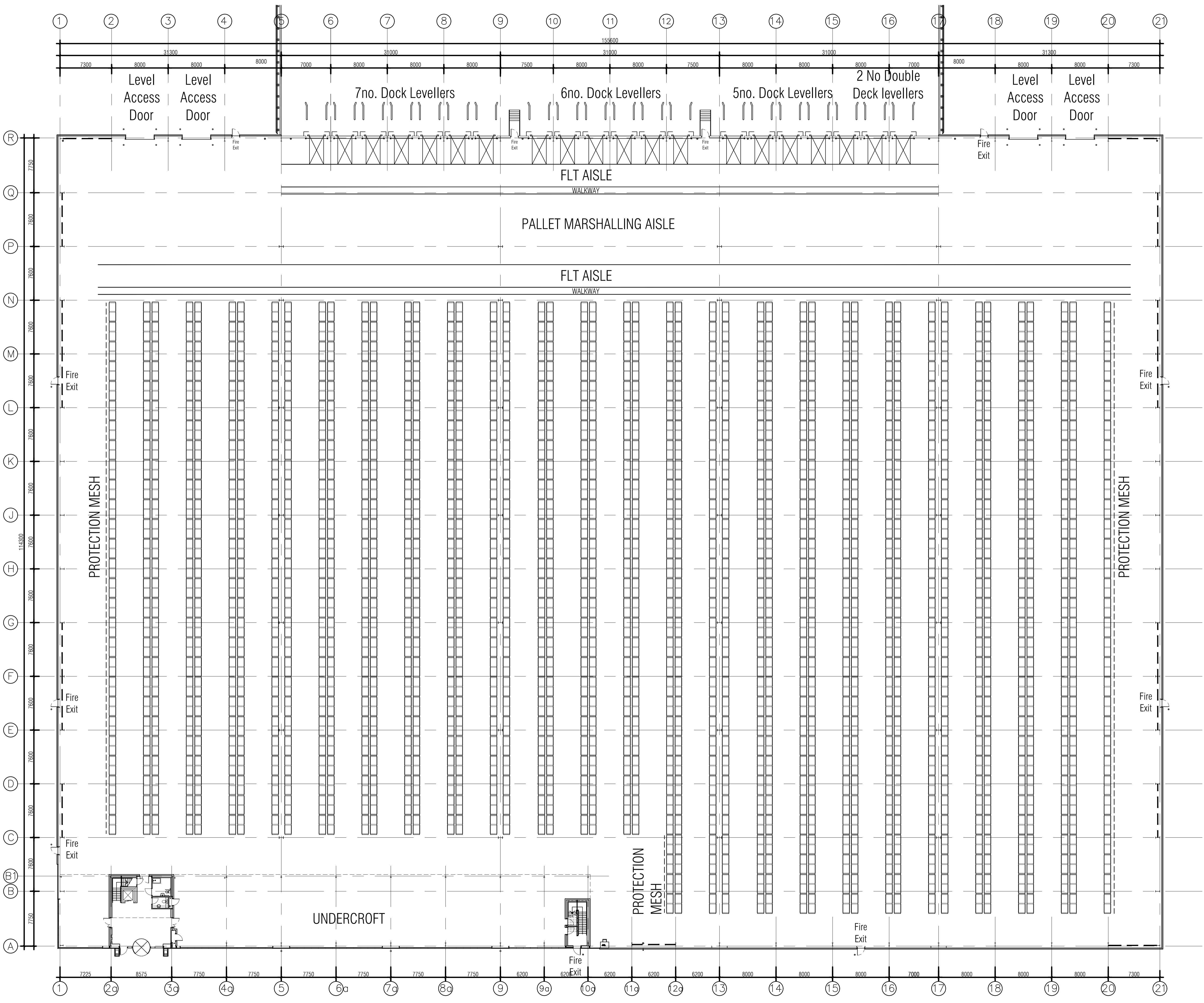
WIDE AISLE PALLET RACKING SETTING OUT 1:20
