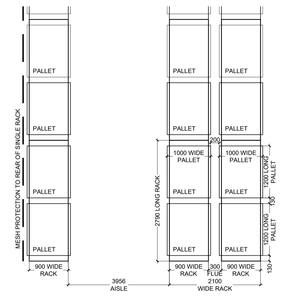
WIDE AISLE PALLET RACKING SETTING OUT 1:20
